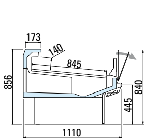
VDB SELF riserva/storage
