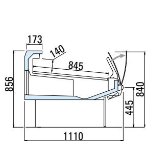
VCB SELF riserva/storage
