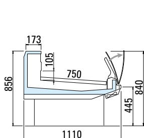
VCB SELF FH
