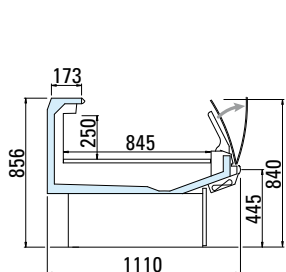
VCB MAXI SELF
